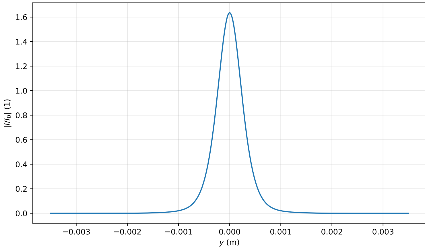
Intensity profile I(x=0, y, z=2.149)/I_0 , P_{in}=0.9P_{cr} , artificial time
